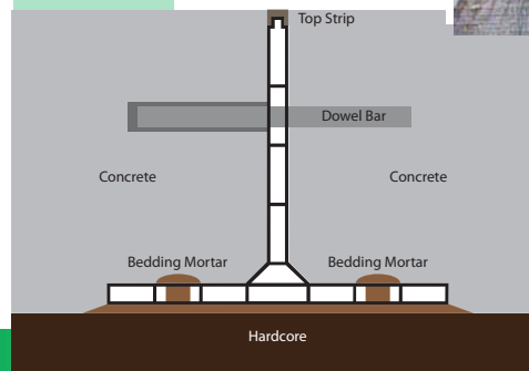
Cross Section of K-FORM.
